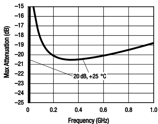
Figure 12. 20 dB State vs Frequency (Bypass Capacitor = 100 pF, Blocking Capacitor = 220 pF, Bypass Resistor = 15 \Omega )
