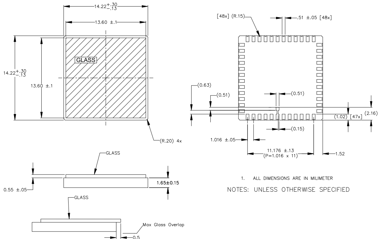
Figure 42. Package Drawing for the 48-pin LCC Package
