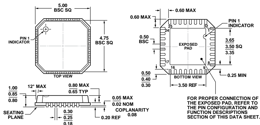
COMPLIANT TO JEDEC STANDARDS MO-220-VHHD-2 Figure 26. 32-Lead Lead Frame Chip Scale Package [LFCSP_VQ] 5 mm × 5 mm Body, Very Thin Quad (CP-32-4) Dimensions shown in millimeters
