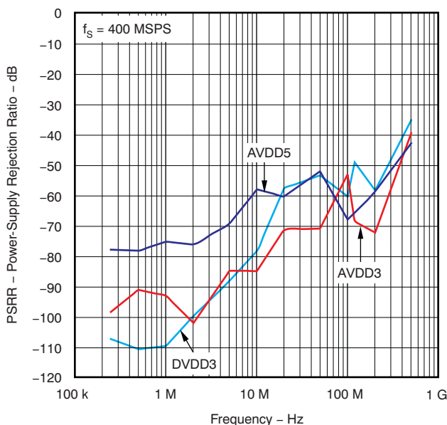
Figure 49. PSRR versus Supply Injected Frequency
