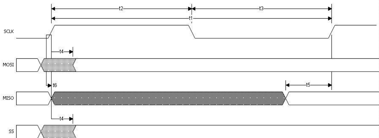
Figure 5-9 Typical SPI Master Timing
