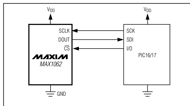
Figure 12a. SPI Interface Connection for a PIC16/PIC17
