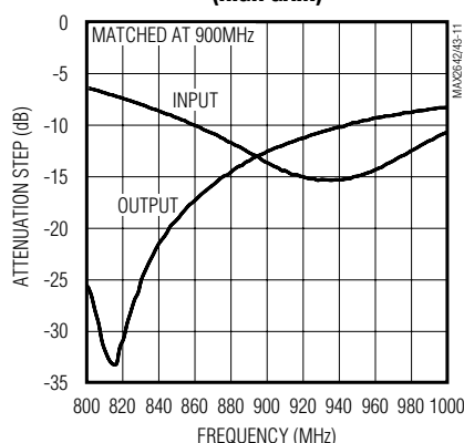
MAX2642 HIGH/LOW-GAIN SWITCH CHARACTERISTICS
