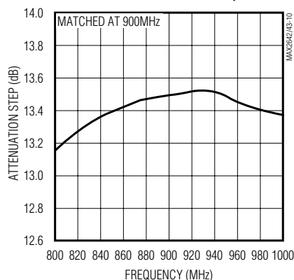
MAX2642 ATTENUATION STEP vs. FREQUENCY
