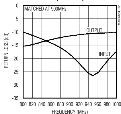
MAX2642 RETURN LOSS vs. FREQUENCY (LOW GAIN)
