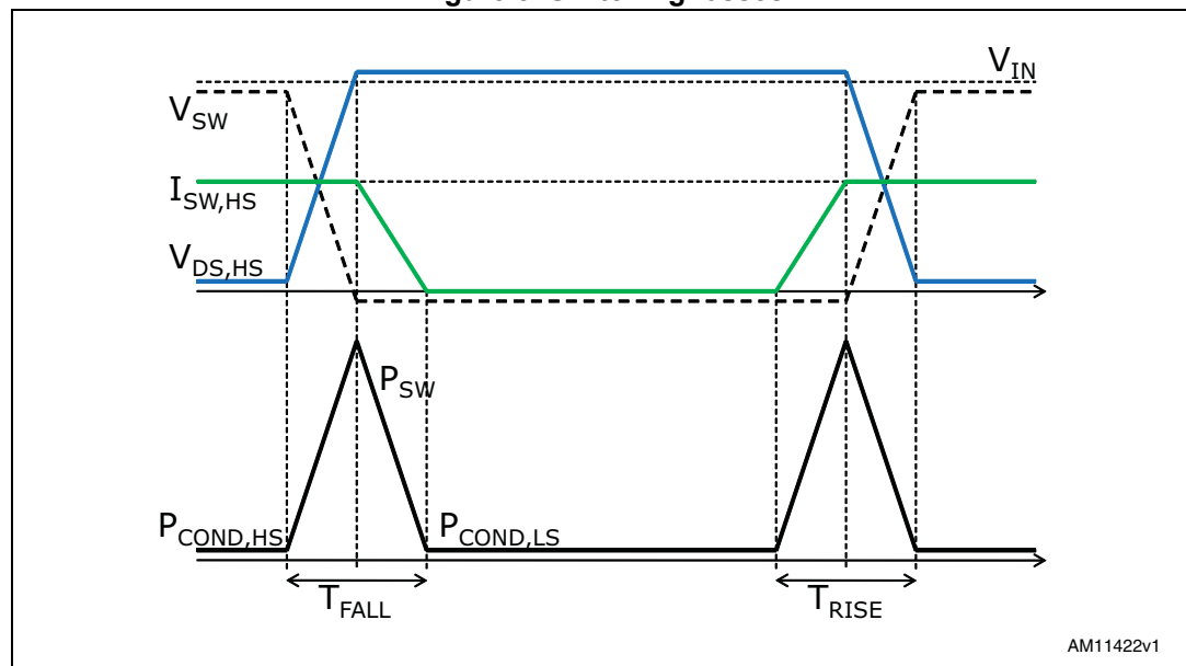
Figure 8. Switching losses
