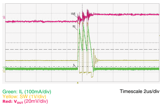
Figure 17. 100 mA operation
