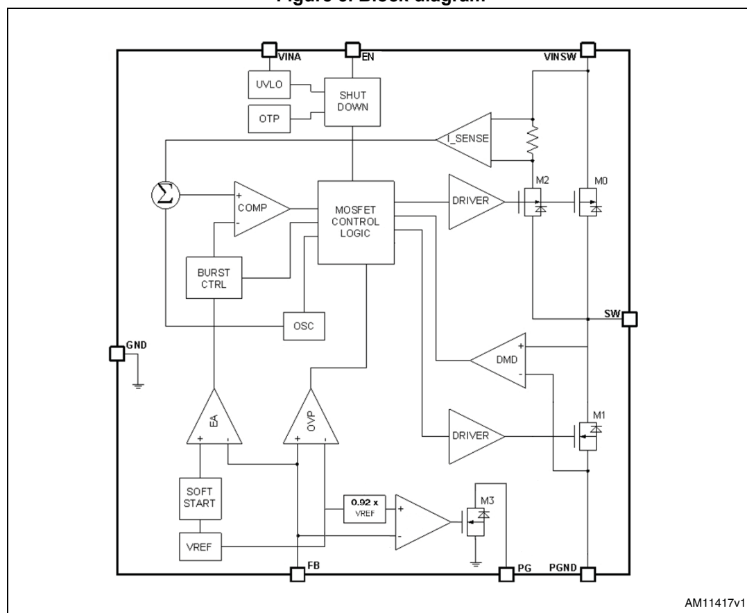
Figure 3. Block diagram
