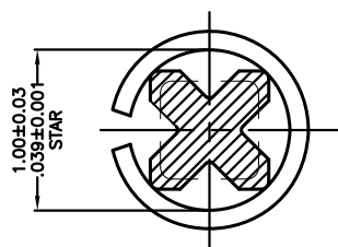
SECTION B-B SCALE 50:1
