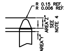
DETAIL Q SCALE 50:1
