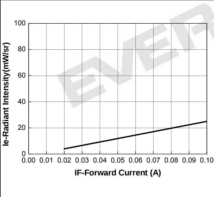
Radiant Intensity vs. Forward Current
