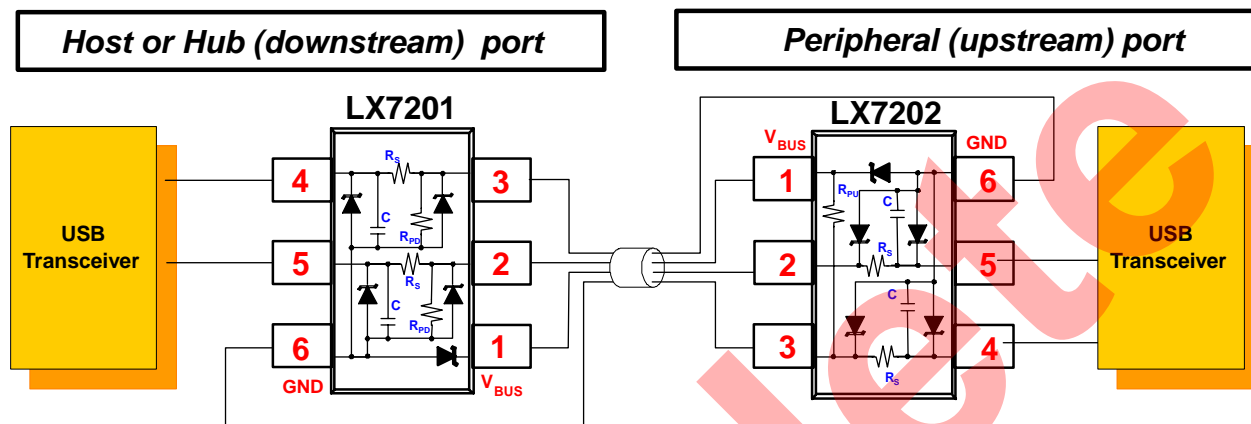
Figure 1 – Typical Application
