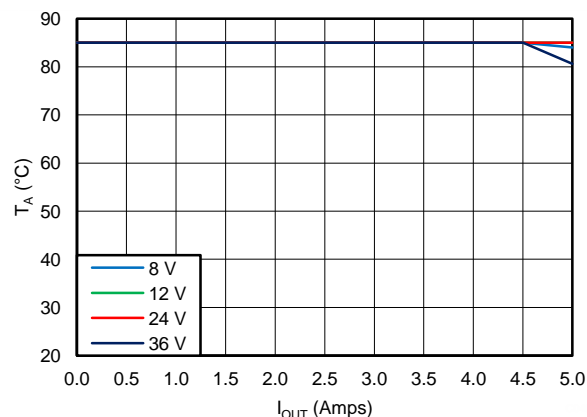
Figure 56. 5V Outputs
