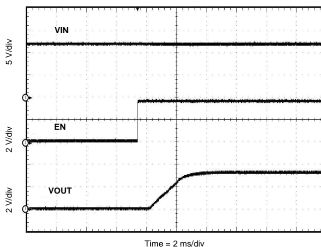
Figure 38. Start-up With EN
