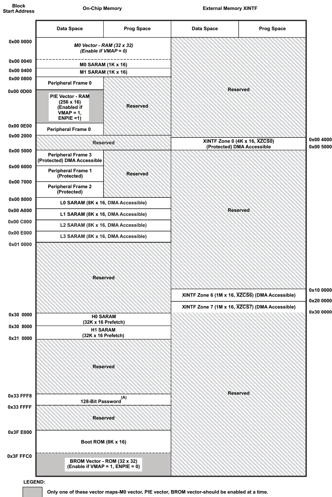
Figure 3-4. C28342, C28341 Memory Map
