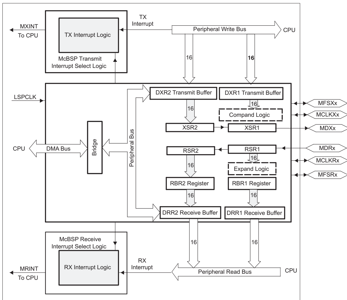
Figure 4-9. McBSP Module
