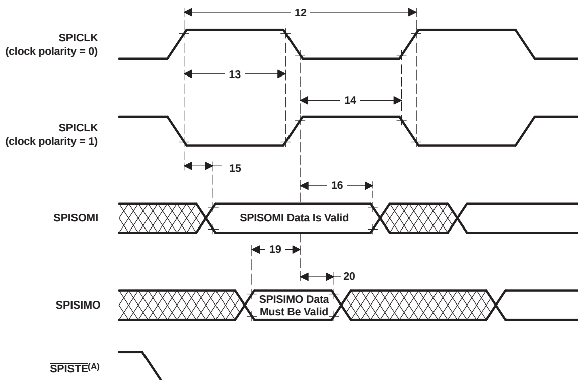
Figure 6-19. SPI Slave Mode External Timing (Clock Phase = 0)
