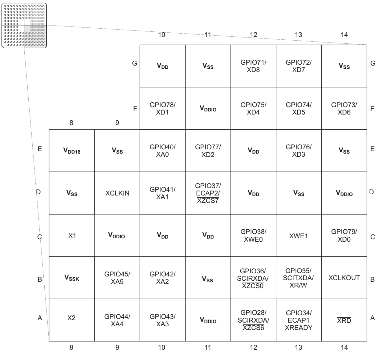
Figure 2-4. C2834x 179-Ball ZHH MicroStar BGA™ Lower Right Quadrant (Bottom View)
