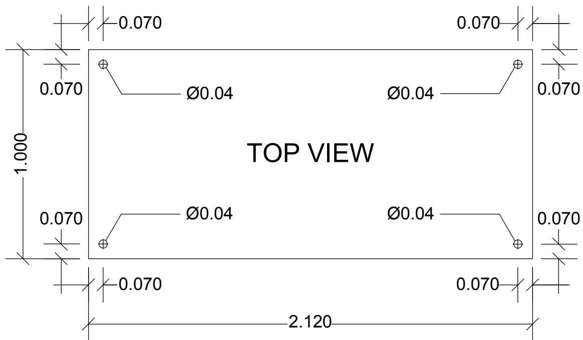
Figure 2.2 EVB-LAN9500A-LC Mechanicals
