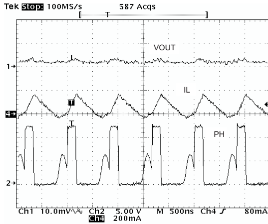
Figure 44. Output Ripple, DCM
