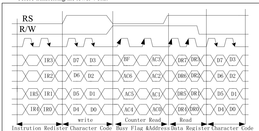
Fig 4-biti transfer Example (M68)
