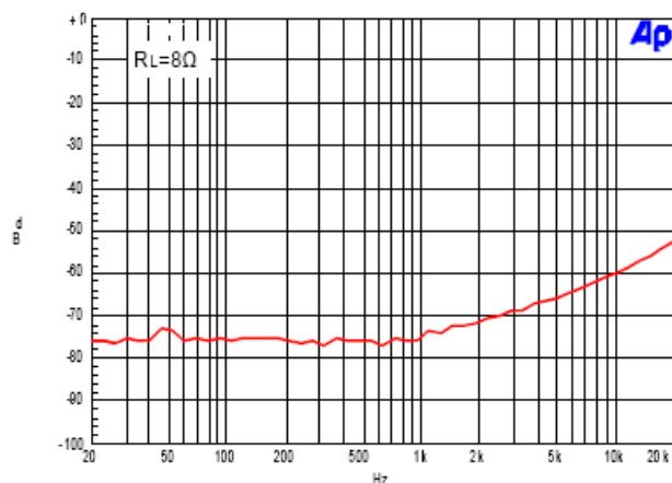
9. PSRR VS Frequency
