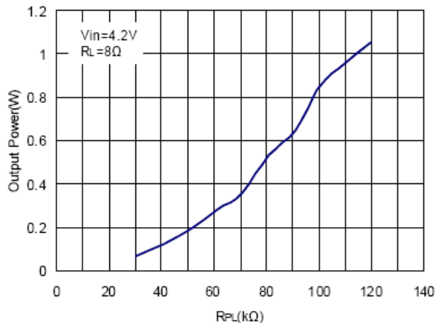
12. RPL VS Output Power
