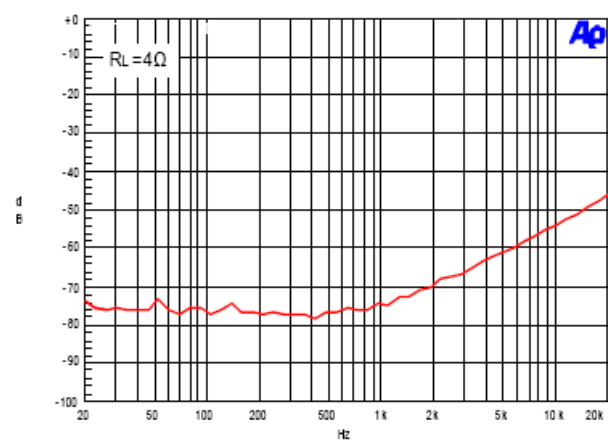
10. PSRR VS Frequency
