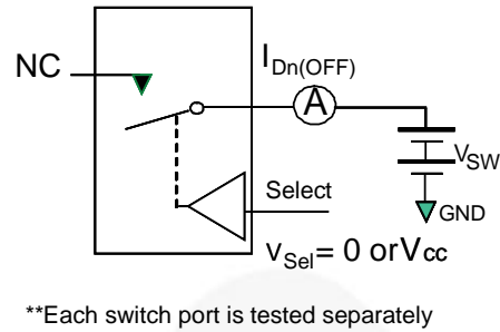
Figure 4. Off Leakage
