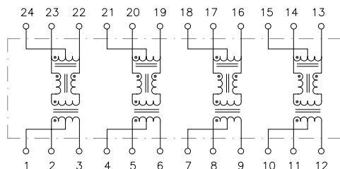
Circuit D
