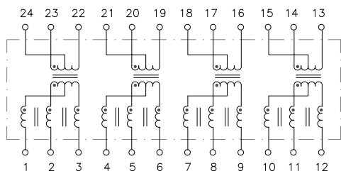
J24 Package
