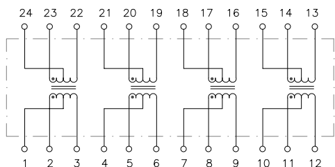
NZ Package
