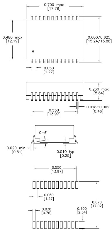
NZ Package
