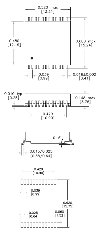
J24 Package
