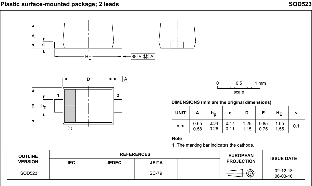
Fig 5. Package outline SOD523
