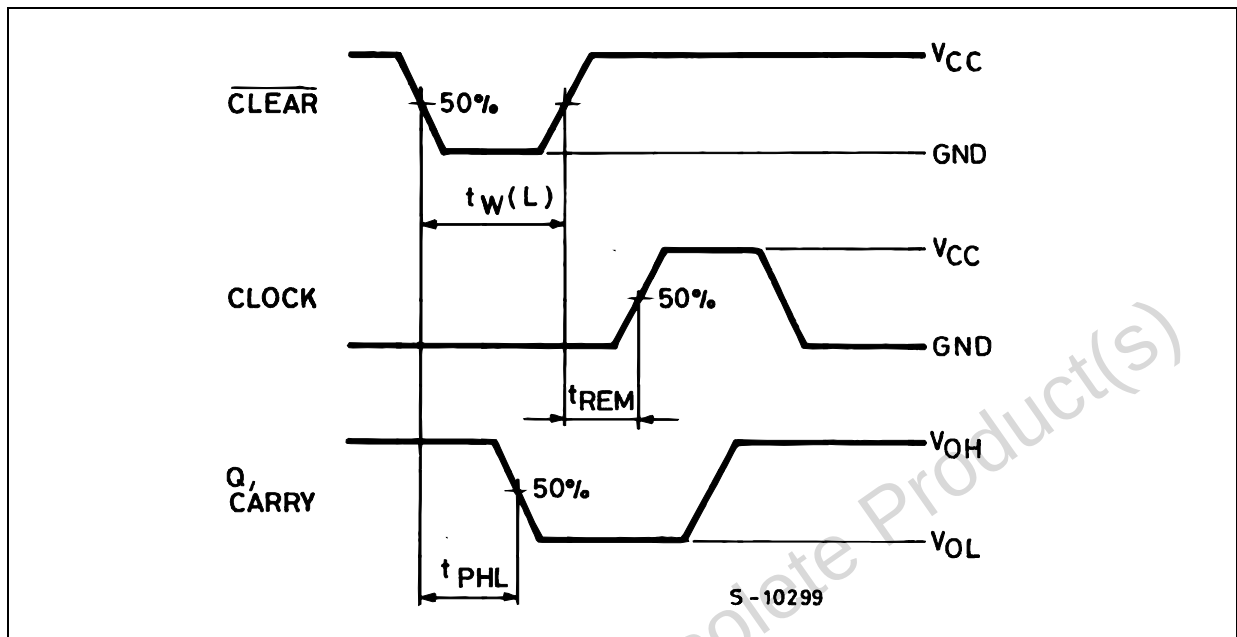
WAVEFORM 2 : PROPAGATION DELAY TIMES, \overline{\text{CLEAR}} MINIMUM PULSE WIDTH (CLEAR MODE) ( f=1\text{MHz} ; 50% duty cycle)
