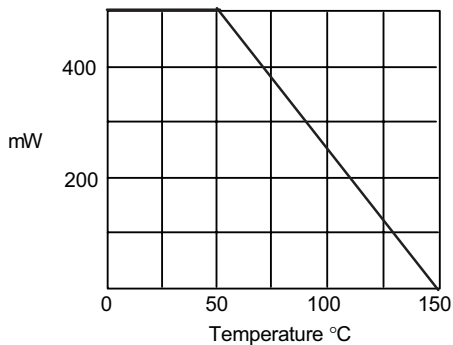
Figure 2 - Derating Curve
