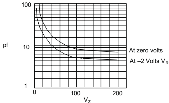
Figure 1 - Typical Capacitance
