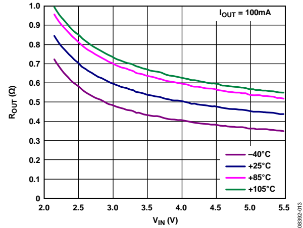
Figure 14. Typical R_{OUT} ( G = 1x ) vs. V_{IN}
