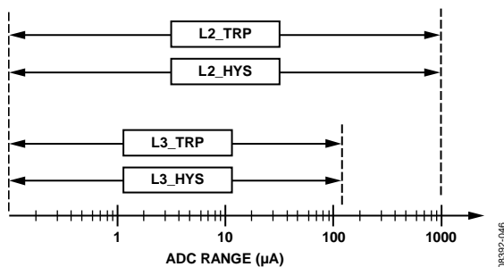
Figure 42. Comparator Ranges
