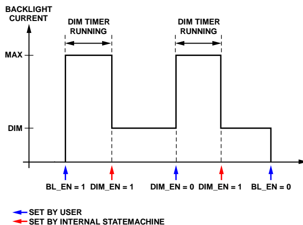
Figure 36. Dim Timer
