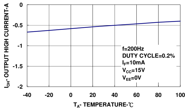
Figure 3: Output High Current vs. Temperature
