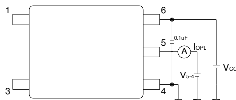
Figure 16 : IOPL test circuit
