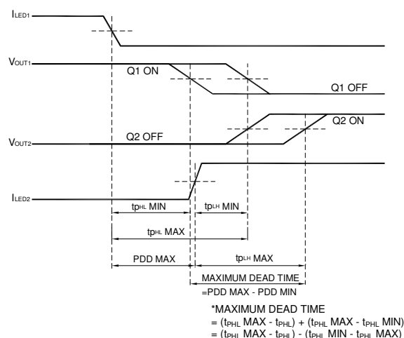
Figure 27 : Waveforms for dead time
