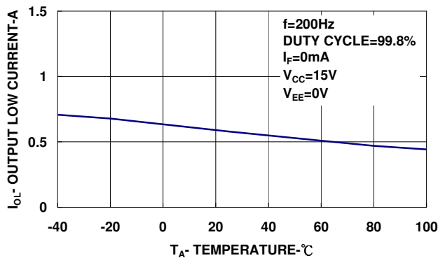
Figure 4: Output Low Current vs. Temperature
