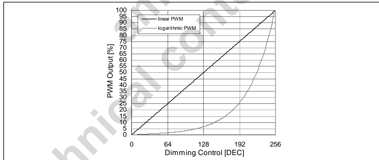
Figure 24. Logarithmic vs. Linear Dimming
