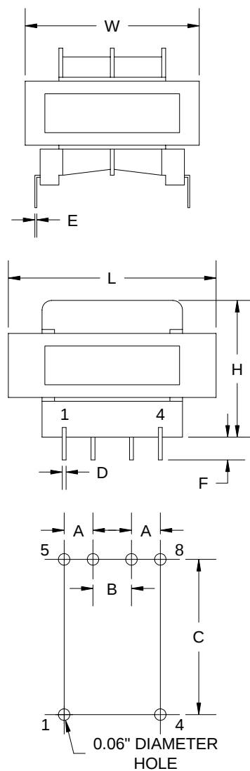
Board Layout
