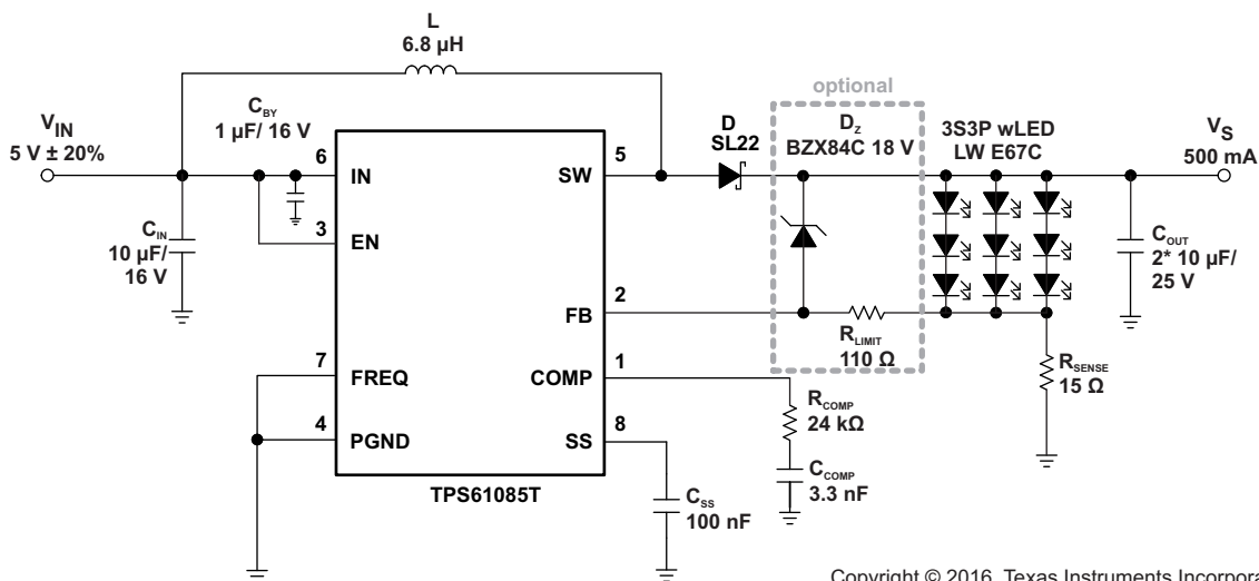
Figure 19. Simple Application (3.3-V Input – f_{sw} = 650 kHz) for wLED Supply (3S3P) (With Optional Clamping Zener Diode)
