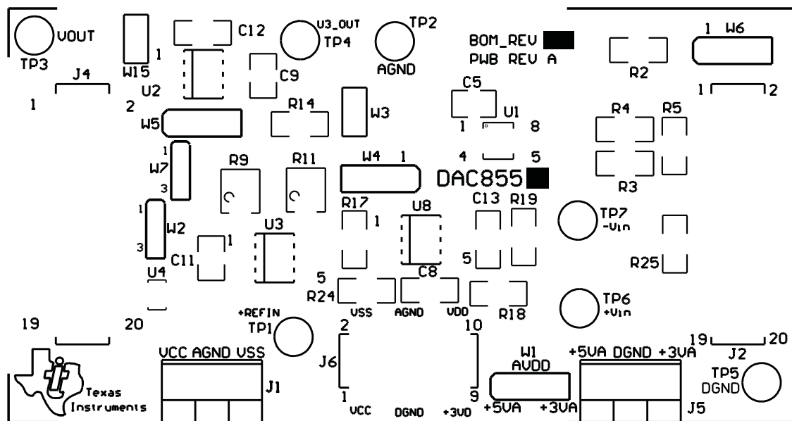
Figure 2. Top Silkscreen
