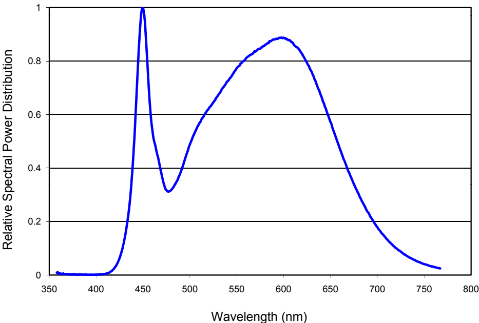
Figure 7. Color spectrum of LXH8-PW40 emitter, integrated measurement.
