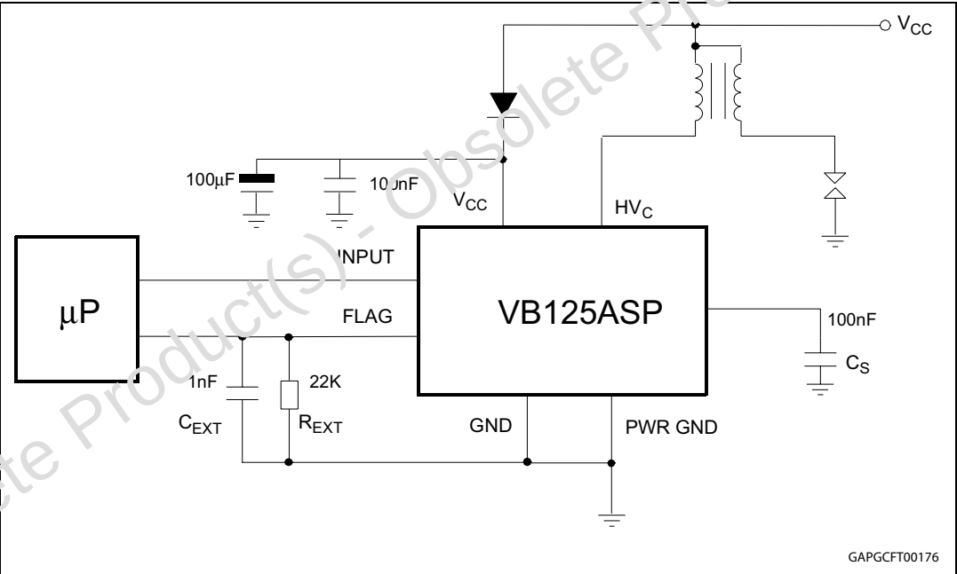
Figure 9. Application circuit
