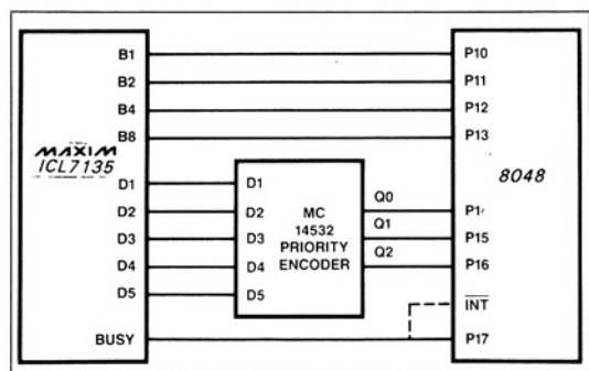
Figure 13. \mu P Interface
