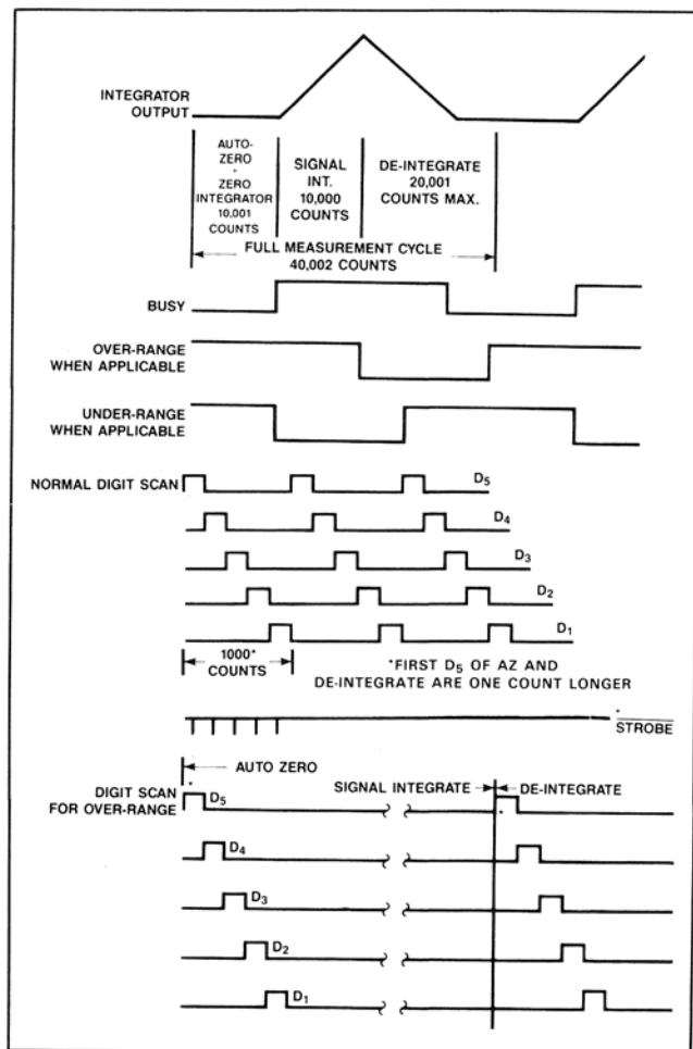
Figure 4. Timing Diagram
