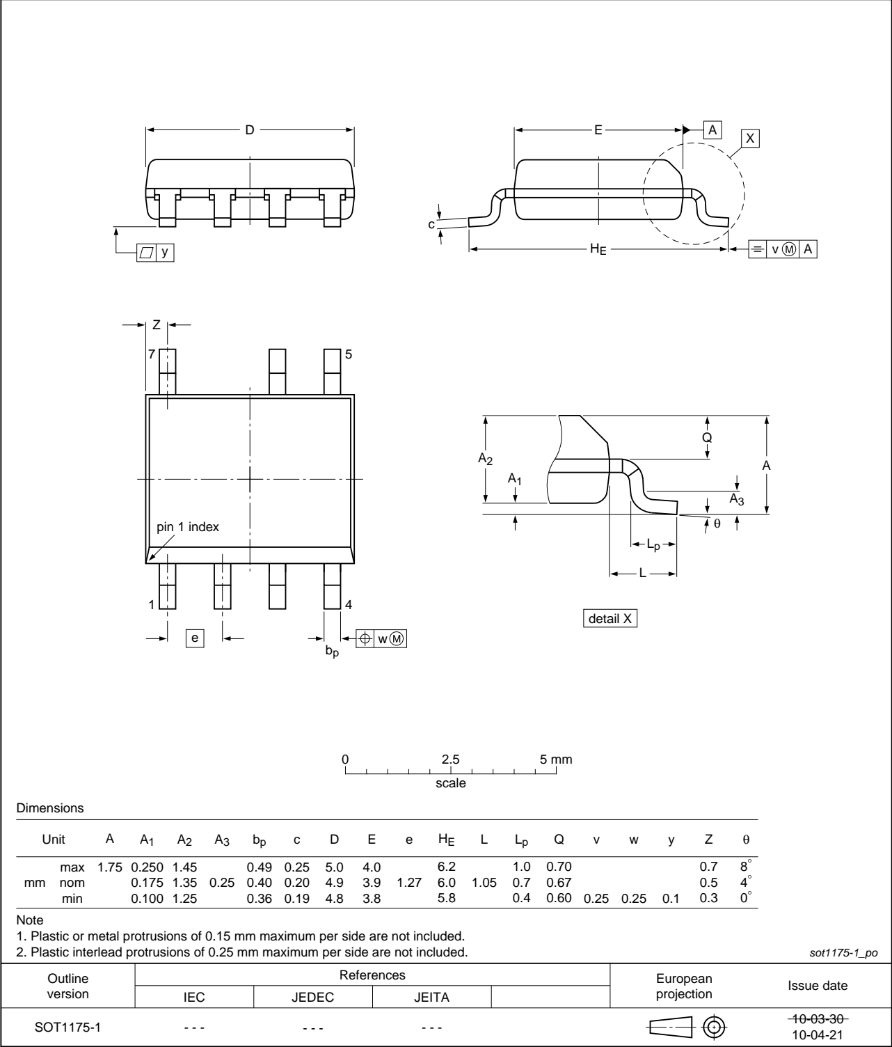
Fig 3. Package outline SOT1175-1 (S07)
