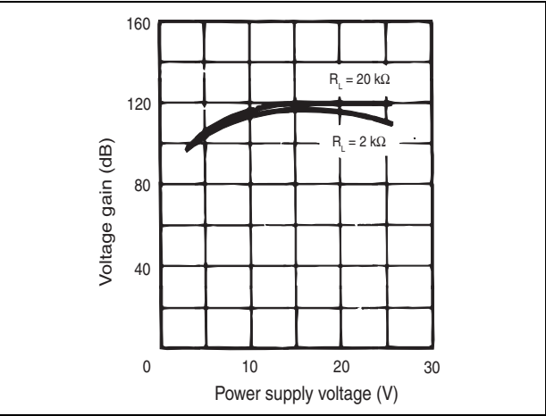
Figure 18. Voltage gain
