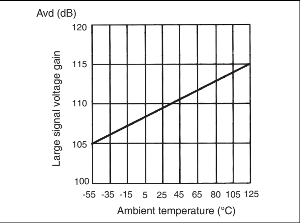
Figure 18. Voltage gain
