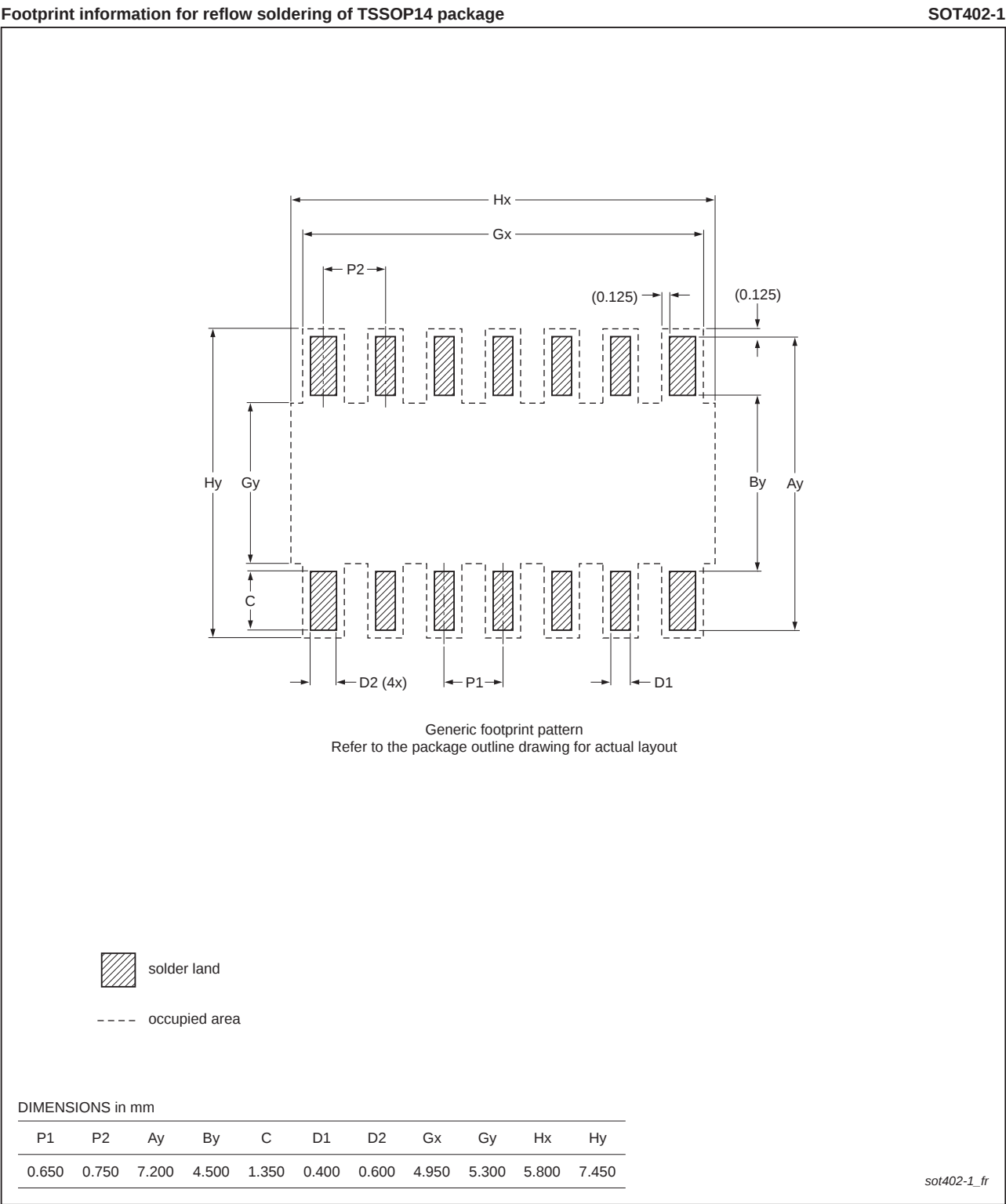
Fig 41. Footprint information for reflow soldering of SOT402-1 (TSSOP14) package of PCF2123TS/1
