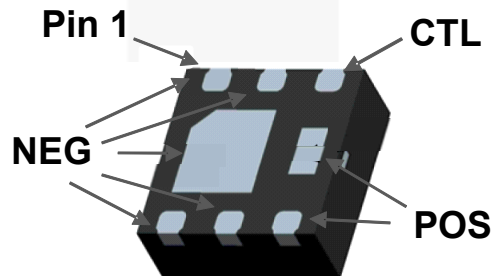
Figure 3. Pin Assignments
