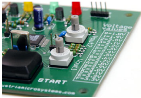
Figure 3: Voltage Selectors
