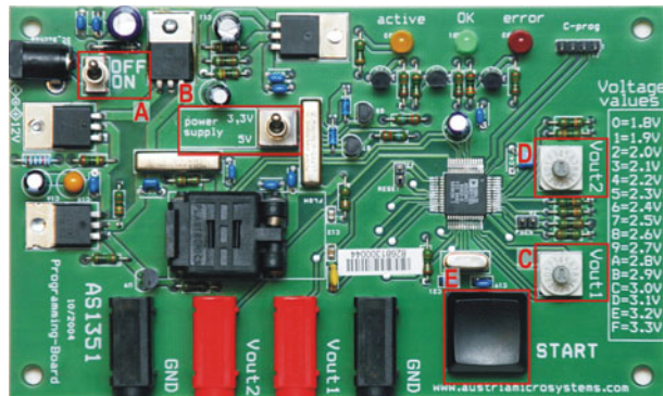
Figure 1: Board description
