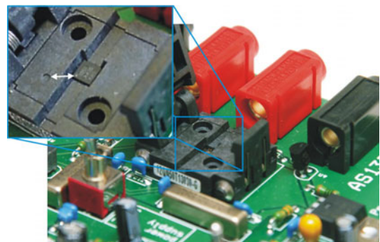
Figure 4: Pin1 Marker
