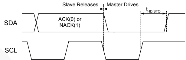
Figure 47. Stop Bit
