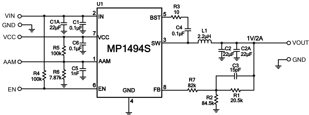
Figure 12: 12V IN , 1V/2A Output
