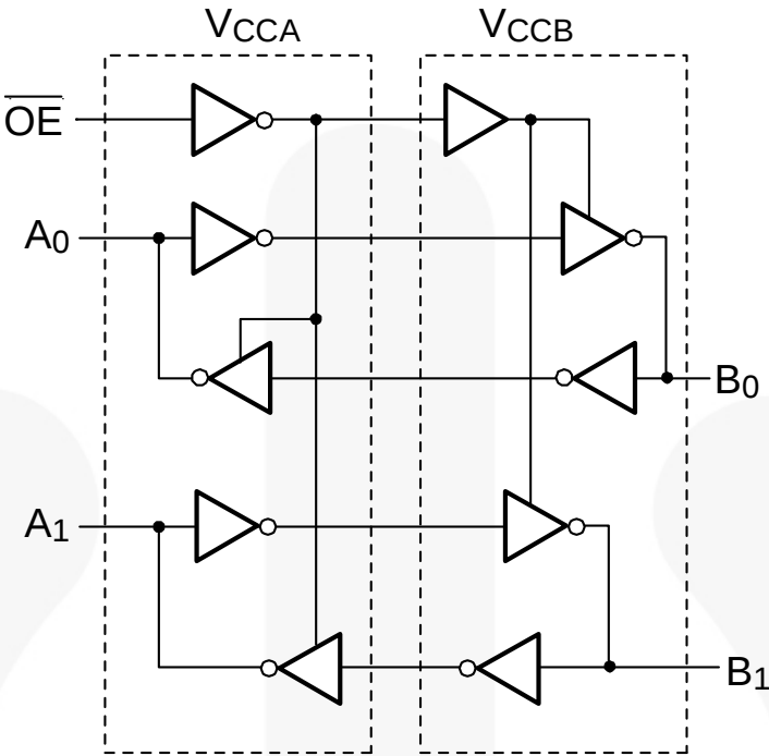
Figure 2. Functional Diagram
