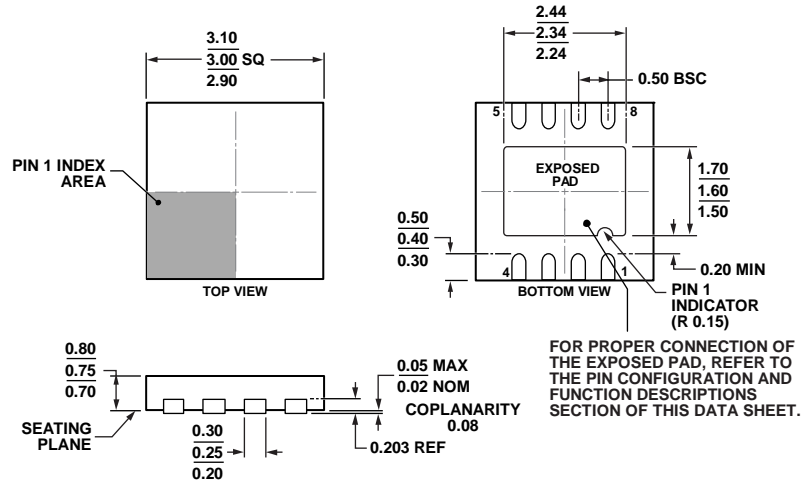
Figure 55. 8-Lead Lead Frame Chip Scale Package [LFCSP_WD] 3 mm × 3 mm Body, Very Very Thin, Dual Lead (CP-8-11) Dimensions shown in millimeters
