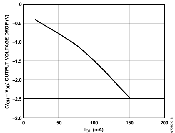
Figure 9. Typical V_{OH} Drop vs. I_{OH} ( V_{DD1} = 5 V, V_{DD1} , V_{ISO} = 12 V to 18 V)
