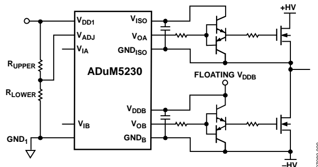
Figure 25. Application Circuit
