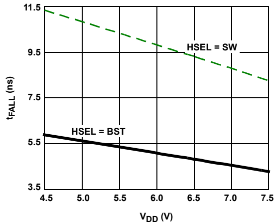
FIGURE 24. HIGH-SIDE DRIVER FALL TIME, t_{FH} (CGH = 3nF, T_A = +25^\circ\text{C} )
