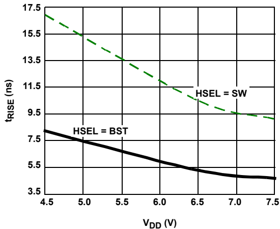
FIGURE 22. HIGH-SIDE DRIVER RISE TIME, t_{RH} (CGH = 3nF, T_A = +25^\circ\text{C} )
