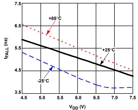
FIGURE 25. t_{FH} WITH TEMPERATURE ( C_{GH} = 3\text{nF} , HSEL = BST)
