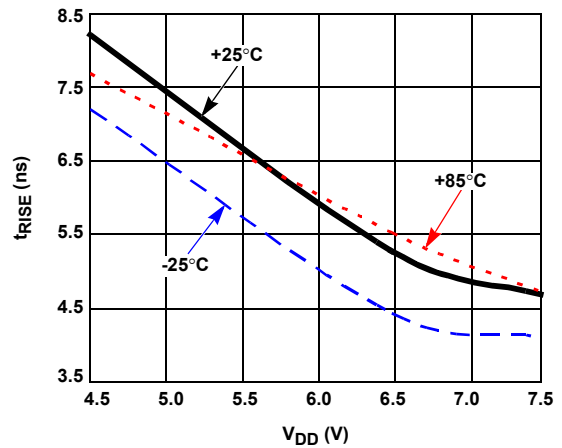
FIGURE 23. t_{RH} WITH TEMPERATURE ( C_{GH} = 3\text{nF} , HSEL = BST)
