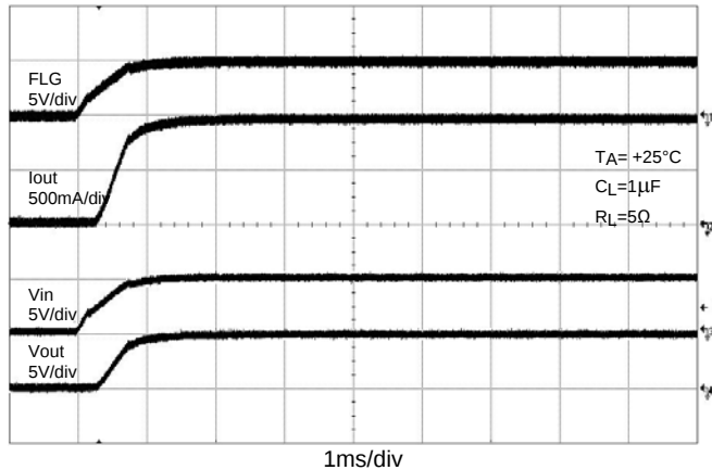
Device Enabled
