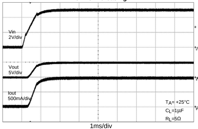
UVLO Increasing
