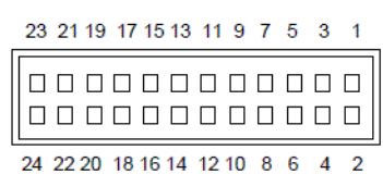
Figure 4-38. PIO Expansion Connector J14
