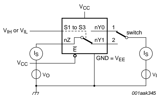
Fig 9. Test circuit for measuring OFF-state leakage current
