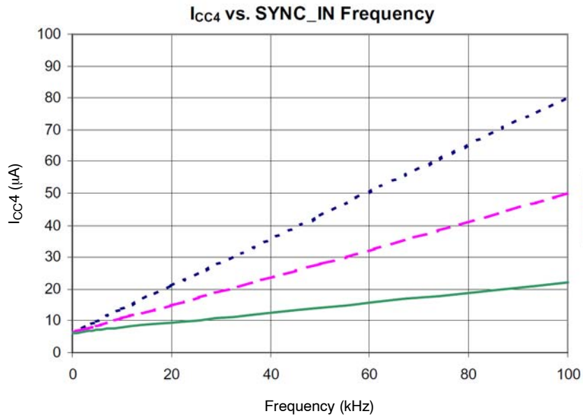
Figure 2. I_{CC4} vs. SYNC_IN Frequency Performance Data
