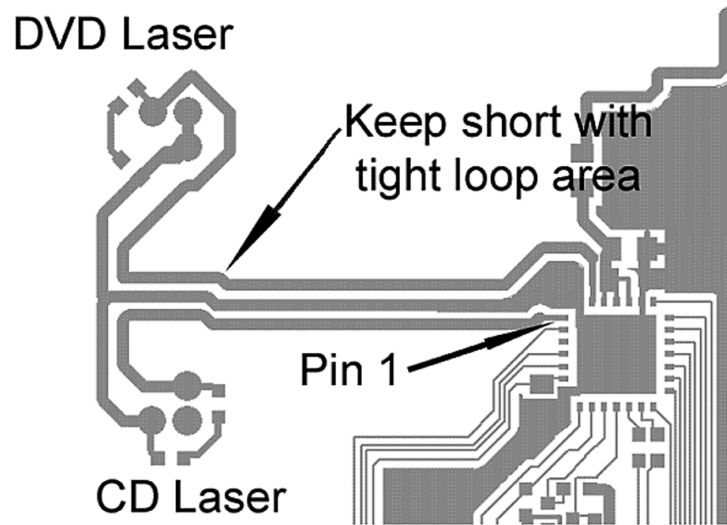
Figure 14. Laser Connection
