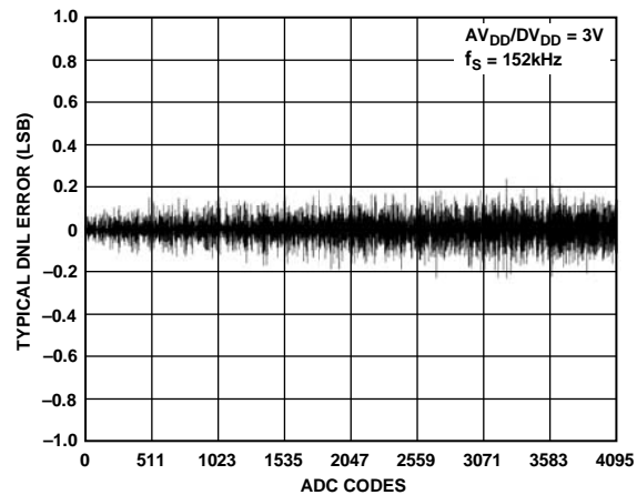
Figure 21. Typical DNL Error, V_{DD} = 3\text{ V}
