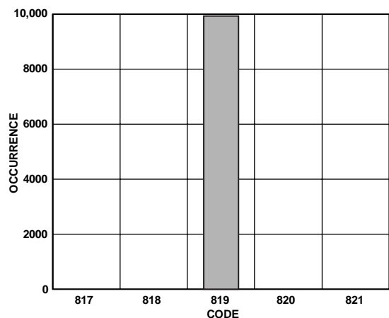
Figure 24. Code Histogram Plot, V_{DD} = 5\text{ V}
