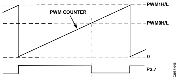
Figure 57. PWM Mode 1
