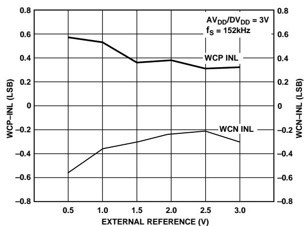
Figure 19. Typical Worst-Case INL Error vs. V_{REF} , V_{DD} = 3\text{ V}
