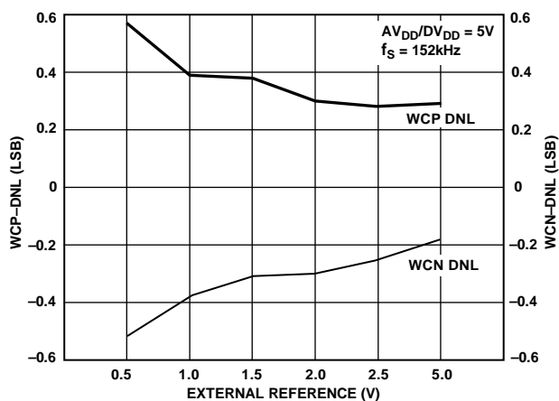
Figure 22. Typical Worst-Case DNL Error vs. V_{REF} , V_{DD} = 5\text{ V}
