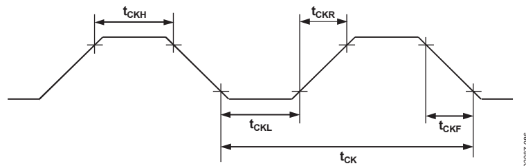
Figure 3. XTAL1 Input
