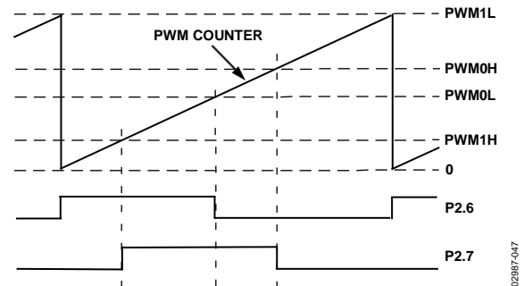
Figure 58. PWM Mode 2
