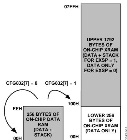
Figure 33. Extended Stack Pointer Operation
