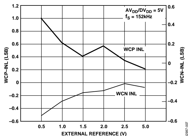
Figure 18. Typical Worst-Case INL Error vs. V_{REF} , V_{DD} = 5\text{ V}
