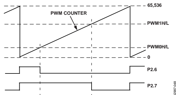
Figure 59. PWM Mode 3
