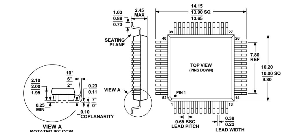
Figure 95. 52-Lead Metric Quad Flat Package [MQFP] (S-52-2)
