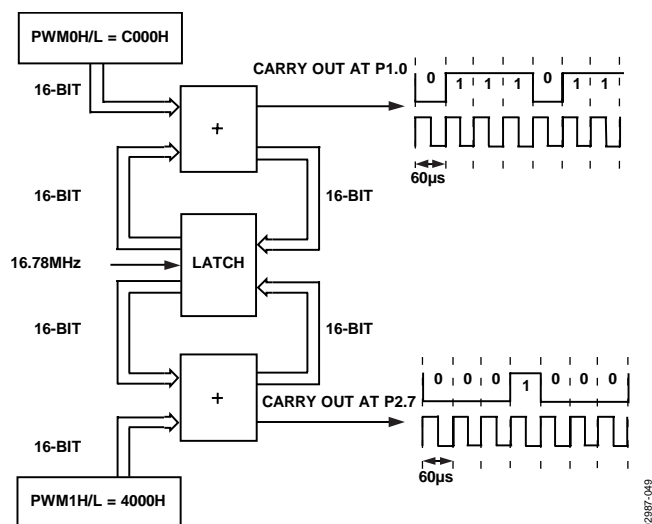
Figure 60. PWM Mode 4
