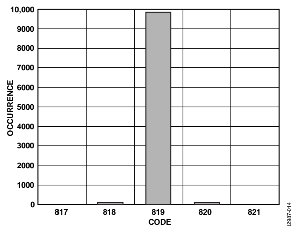
Figure 25. Code Histogram Plot, V_{DD} = 3\text{ V}
