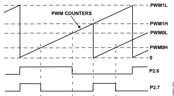
Figure 61. PWM Mode 5
