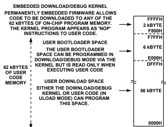
Figure 49. Flash/EE Program Memory Map in ULOAD Mode
