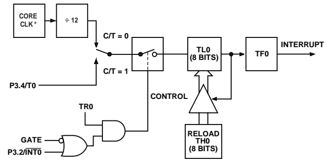
Figure 77. Timer/Counter 0, Mode 2
