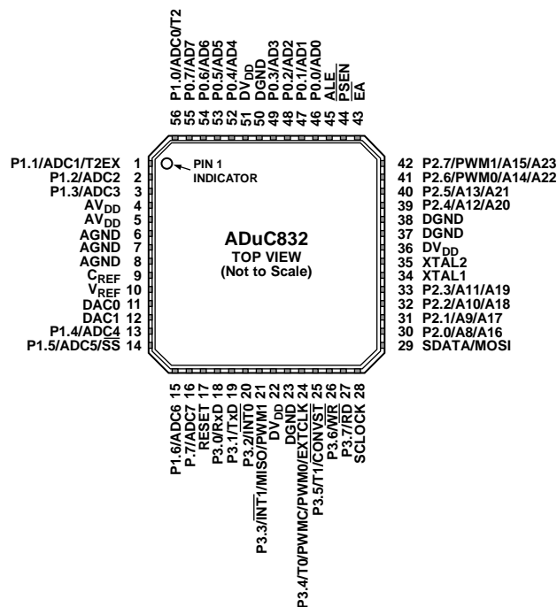
Figure 15. 56-Lead LFCSP
