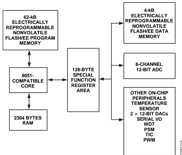
Figure 35. Programming Model
