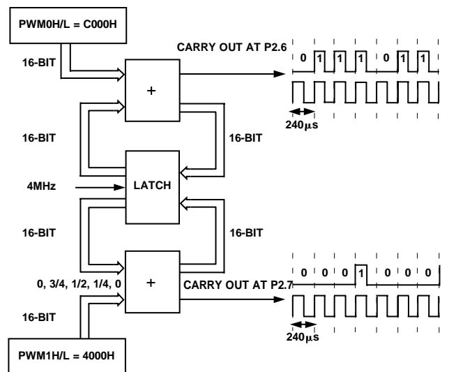
Figure 62. PWM Mode 6
