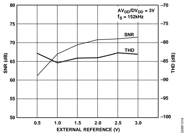
Figure 29. Typical Dynamic Performance vs. V_{REF} , V_{DD} = 3V
