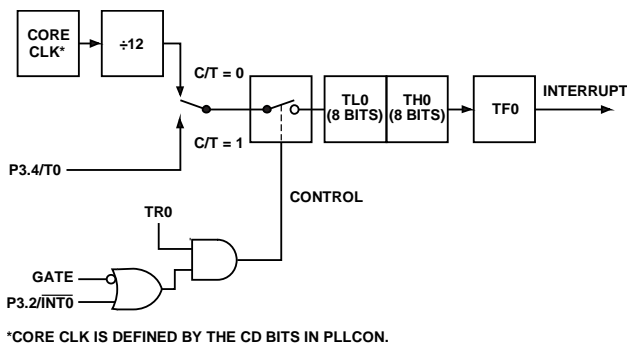
Figure 76. Timer/Counter 0, Mode 1
