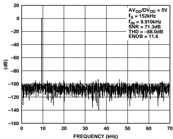
Figure 26. Dynamic Performance at V_{DD} = 5\text{ V}
