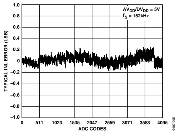
Figure 16. Typical INL Error, V_{DD} = 5\text{ V}
