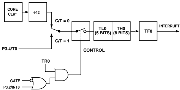
Figure 75. Timer/Counter 0, Mode 0
