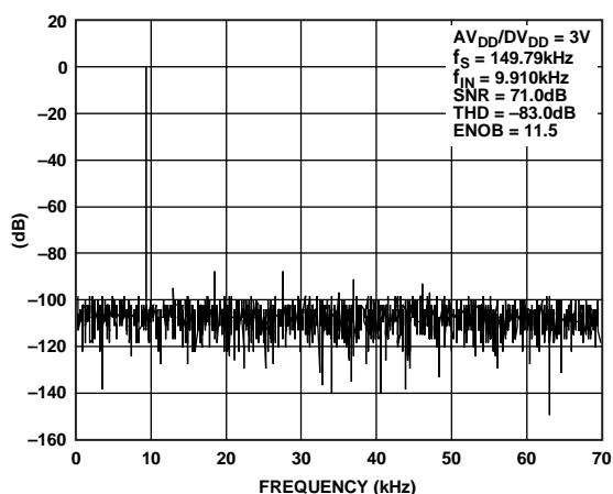
Figure 27. Dynamic Performance at V_{DD} = 3\text{ V}
