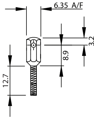
SCREW 6 BA Brass, Nickel Plated
