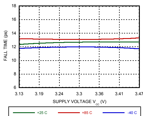
Fall Time vs. Supply Voltage [1][2][3][4]
