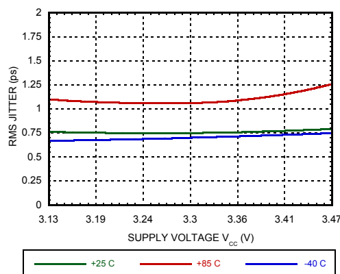
RMS Jitter vs. Supply Voltage [1][2][3][5]
